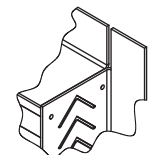
Typical Closed Corner (Optional flanges on all four (4) sides)
