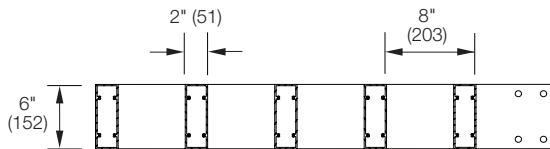
Horizontal Section
