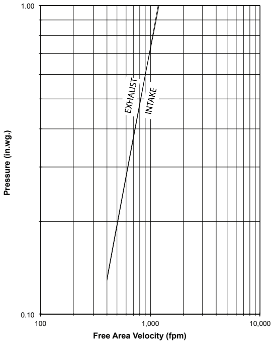
Louver Test Size = 48" x 48" (1219 x 1219) Pressure loss tested in accordance with Figure 5.5 of AMCA Standard 500-L.
